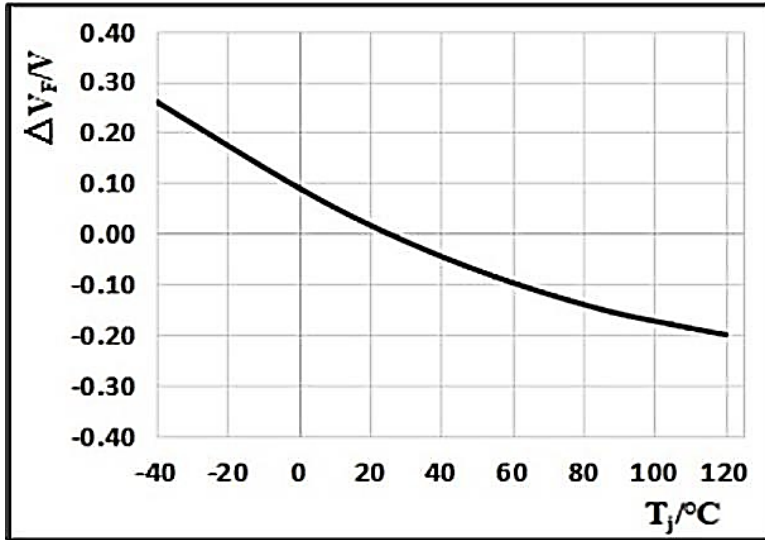
Figure 5. Junction Temperature Vs. \Delta V_F , \Delta V_F = V_F - V_F(25^\circ\text{C}) = f(T_j)
