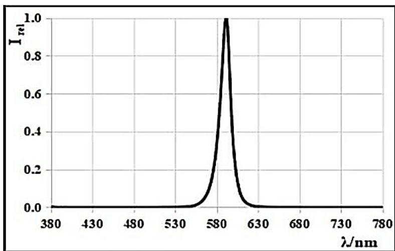
Figure 1. Relative Spectral Emission, I_{rel}=f(\lambda) , \Phi_{rel} = f(\lambda) ; T_j = 25^\circ \text{C} ; IF= 140mA
