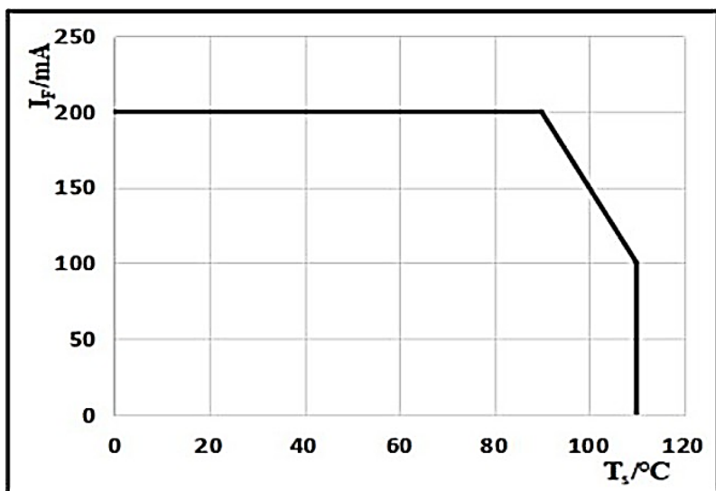
Figure 7 Ts Vs. Max. Permissible IF, I_F = f(T_s)
