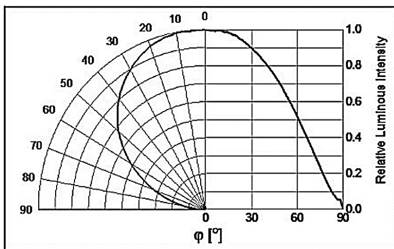
Figure 8. Radiation Diagram, I_{rel} = f(\Phi)
