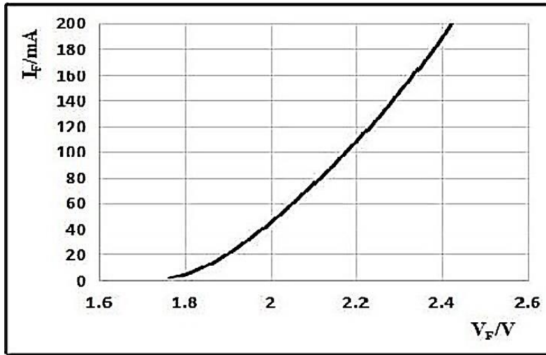
Figure 3. Forward Voltage Vs. Forward Current, IF = f (VF)
