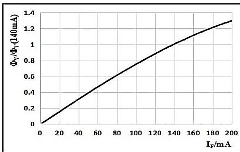
Figure 2. Forward Current Vs. Relative Intensity, \Phi_V/\Phi_V(140\text{mA})= f(I_F)
