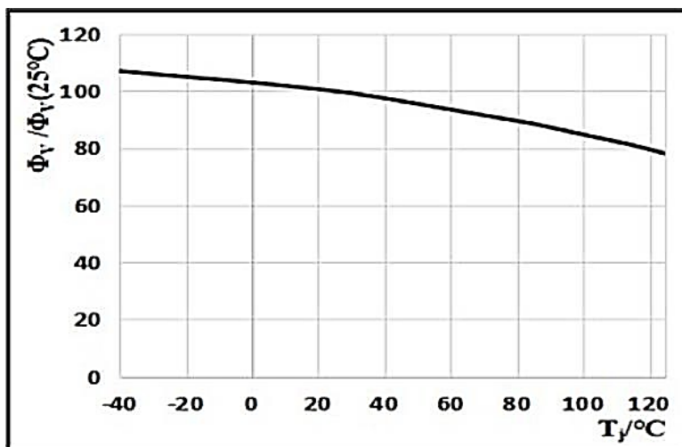
Figure 5. Junction Temperature Vs. Relative Intensity, \Phi_V/\Phi_V(25^\circ\text{C})=f(T_j)
