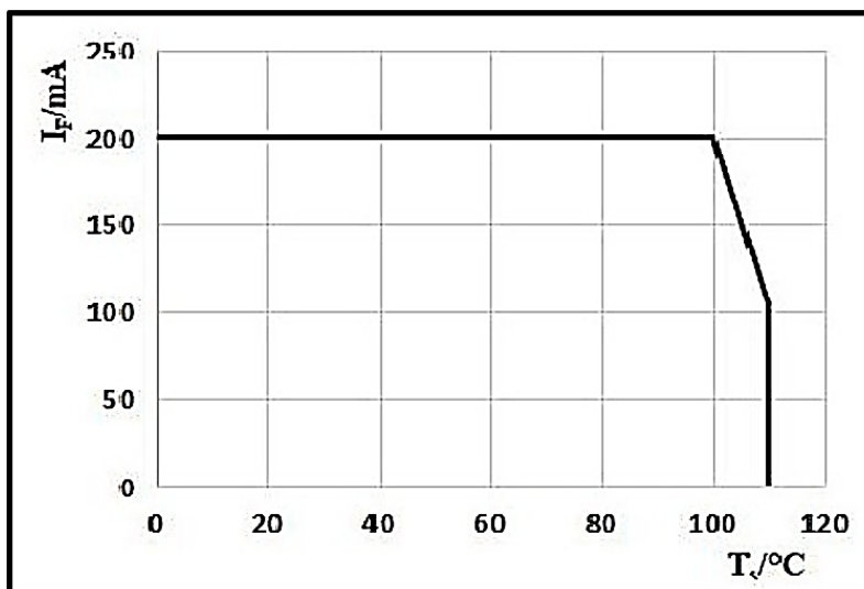
Figure 8 Ts Vs. Max. Permissible IF, I_F = f(T_s)
