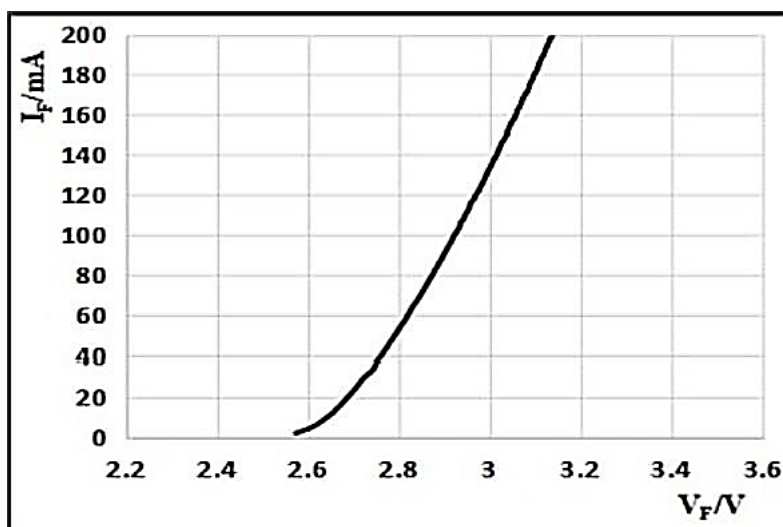
Figure 3. Forward Voltage Vs. Forward Current, I_F = f(V_F)
