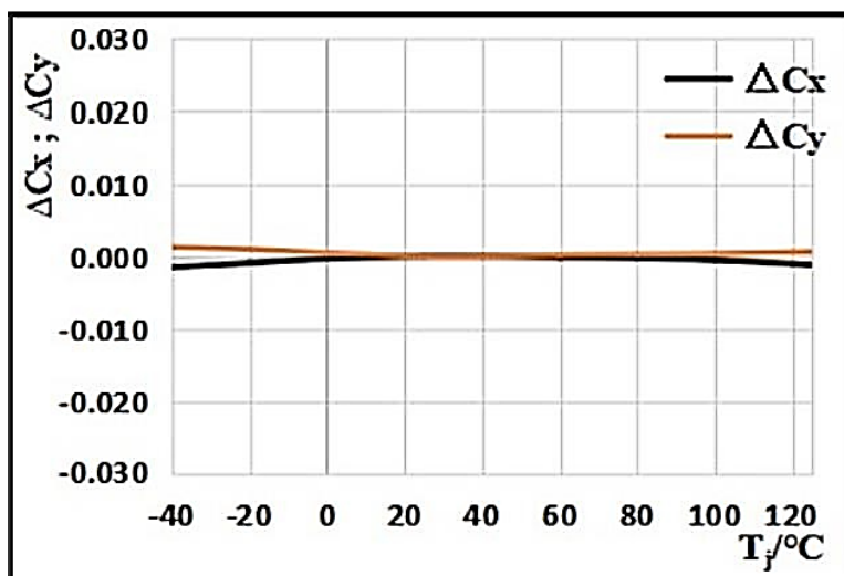
Figure 7. Junction Temperature Vs. Chromaticity Coordinate \Delta C_x , \Delta C_y = f(T_j)
