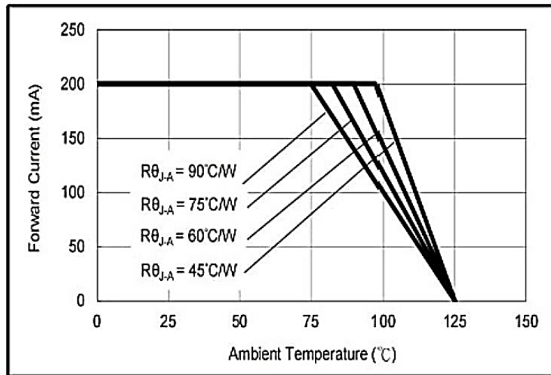
Figure 5 Ts Vs. Max. Permissible IF, IF = f(T_s)
