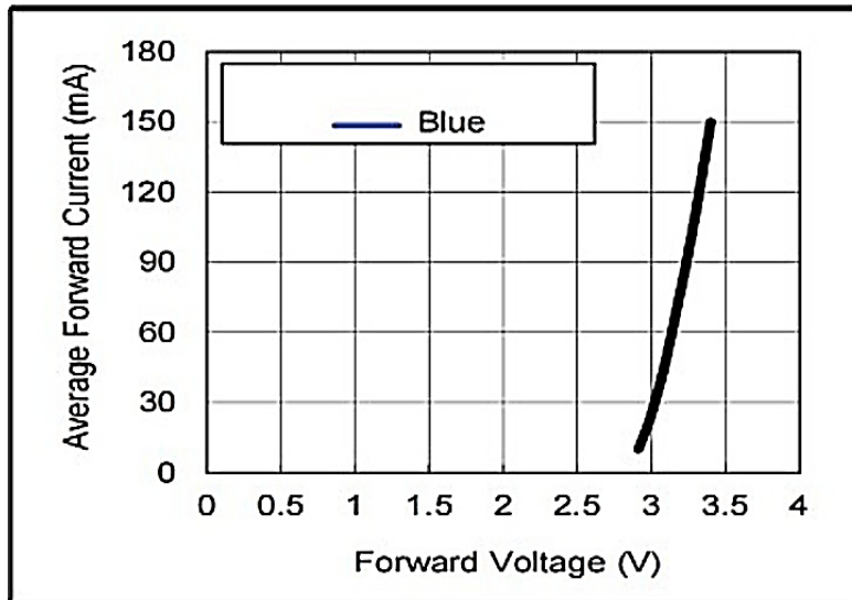
Figure 3. Forward Voltage Vs. Forward Current, IF = f (VF)
