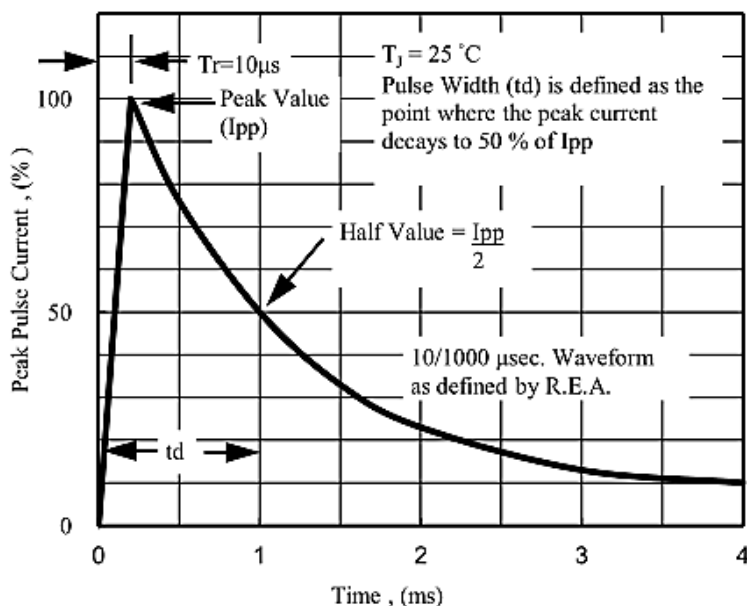
Fig. 5 - Pulse Waveform
