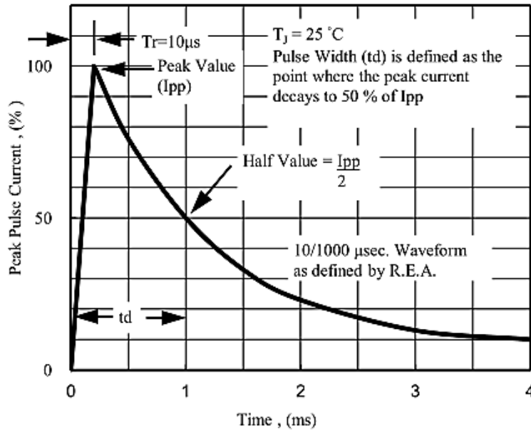
Fig. 5 - Pulse Waveform
