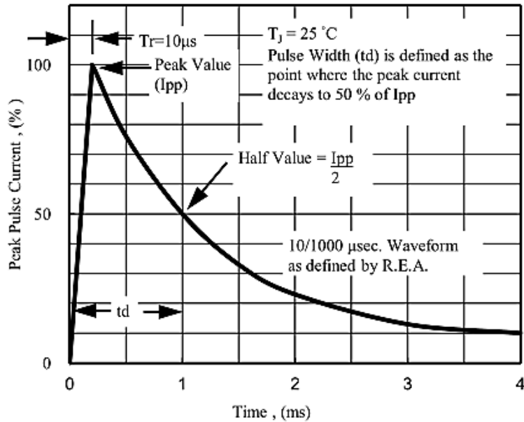
Fig. 5 - Pulse Waveform
