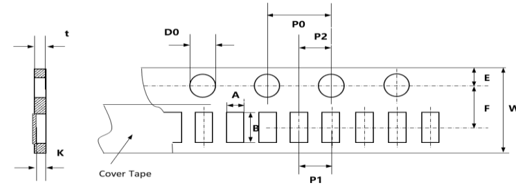
Fig. 7-2 0201 (Paper tape/ 2 mm pitch)
