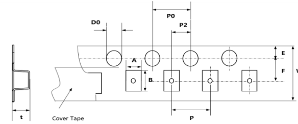
Fig. 7-5 0603, 0805, 1206, 1210, 2220 (Plastic tape)
