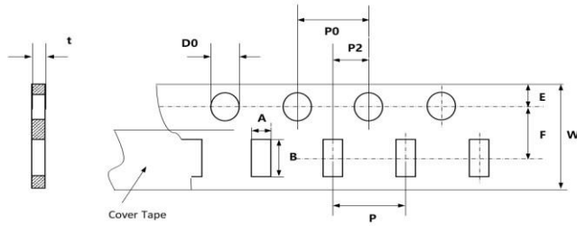
Fig. 7-4 0603, 0805, 1206, 1210, 2220 (Paper tape)
