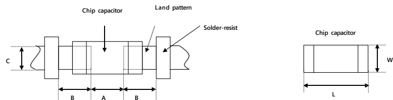
Recommended land dimensions for reflow-soldering
