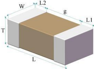
Fig.1 Structure & Dimension
