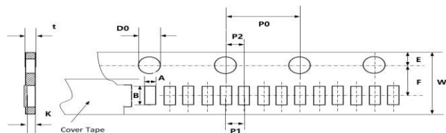
Fig. 7-1 0402 (Paper tape/ 2 mm pitch)
