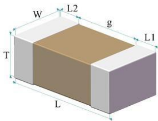
Fig.1 Structure & Dimension
