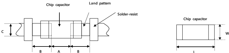
Recommended land dimensions for reflow-soldering (unit: mm)
