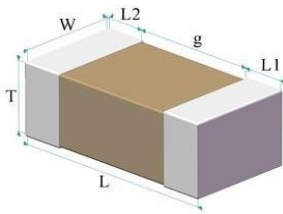
Fig.1 Structure & Dimension
