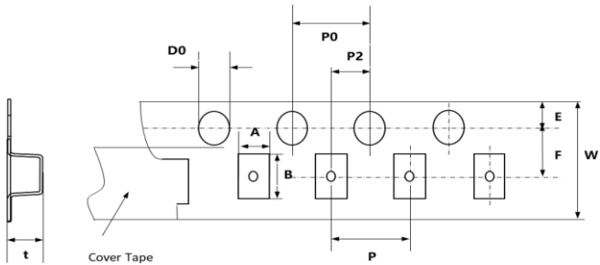
Fig. 5-6 0603 (Plastic tape)
