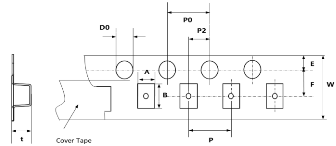
Fig. 5-6 0603 (Plastic tape)
