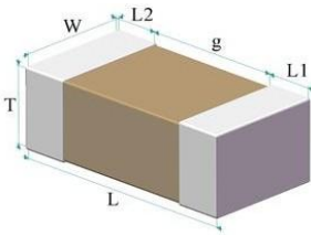
Fig.1 Structure & Dimension
