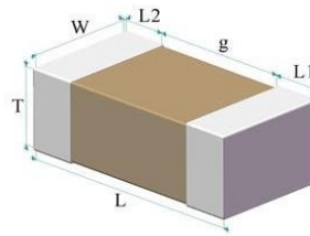
Fig.1 Structure & Dimension
