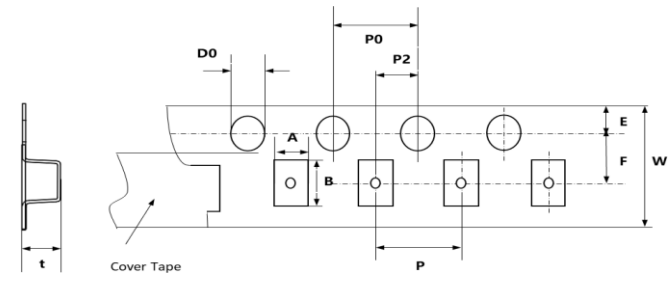
Fig. 7-5 0603,0805,1206,1210 ,2220 (Plastic tape)
