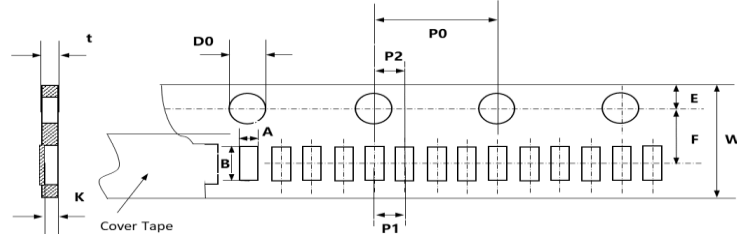
Fig. 5-3 0201 (Paper tape/ 1 mm pitch)
