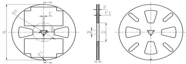
Fig. 6-1 Disc (Width of carrier-4 mm)
