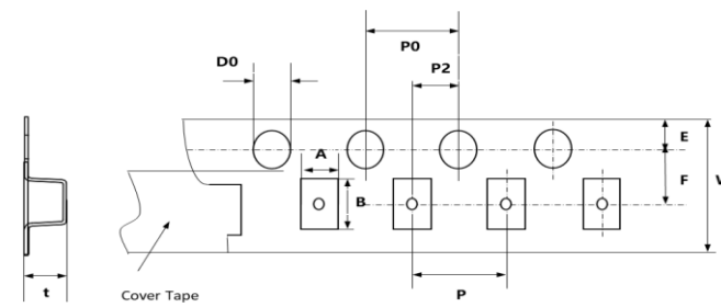
Fig. 7-5 0603,0805,1206,1210 ,2220 (Plastic tape)
