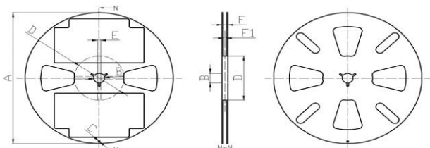
Fig. 8-2 Disc (Width of carrier-16 mm)
