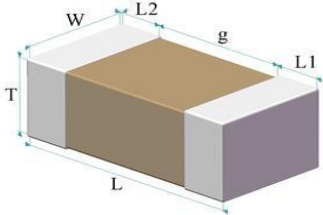
Fig.1 Structure & Dimension
