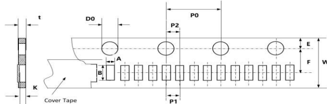
Fig. 7-3 0201 (Paper tape/ 1 mm pitch)
