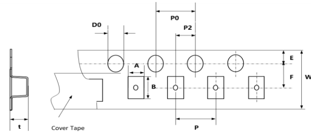
Fig. 7-5 0603 (Plastic tape)
