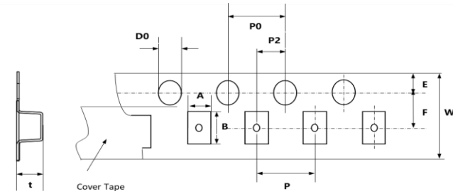
Fig. 7-5 0603 (Plastic tape)
