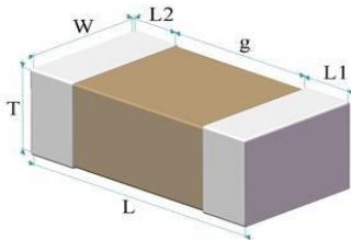
Fig.1 Structure & Dimension
