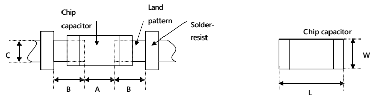
Recommended land dimensions for reflow-soldering
