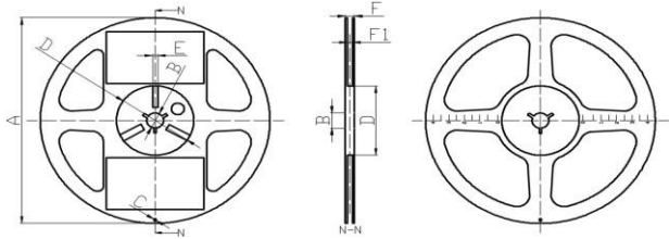
Fig. 6-1 Disc (Width of carrier-8 mm)
