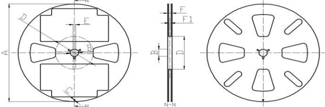
Fig. 6-2 Disc (Width of carrier-16 mm)
