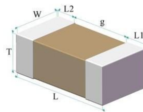
Fig.1 Structure & Dimension
