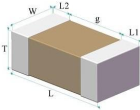
Fig.1 Structure & Dimension
