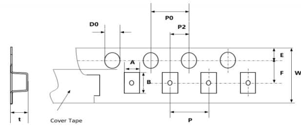
Fig. 5-6 0603,0805,1206,1210 (Plastic tape)
