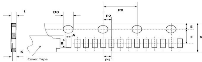
Fig. 5-3 0201 (Paper tape/ 1 mm pitch)
