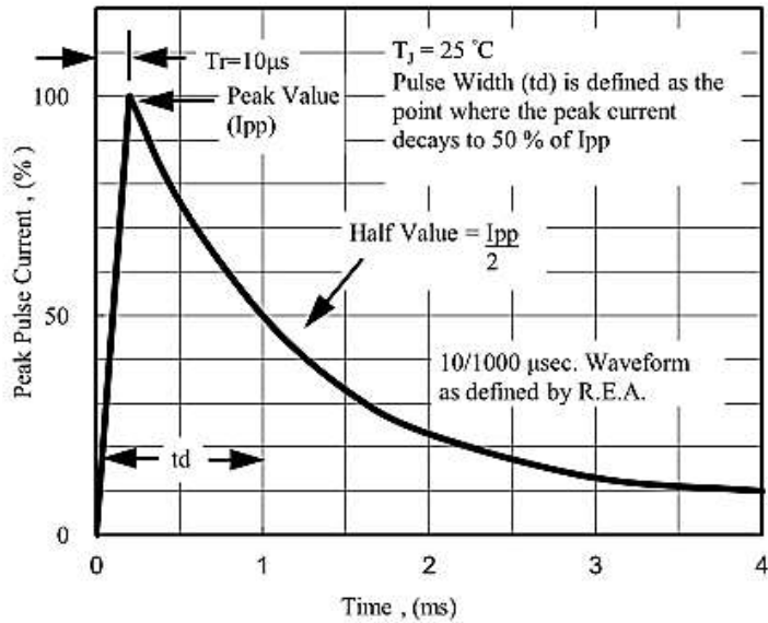
Fig. 5 - Pulse Waveform
