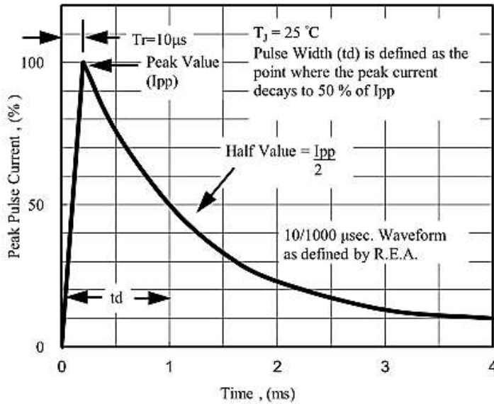
Fig. 5 - Pulse Waveform
