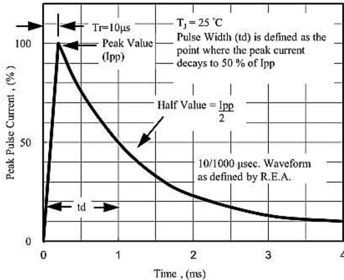
Fig. 5 - Pulse Waveform
