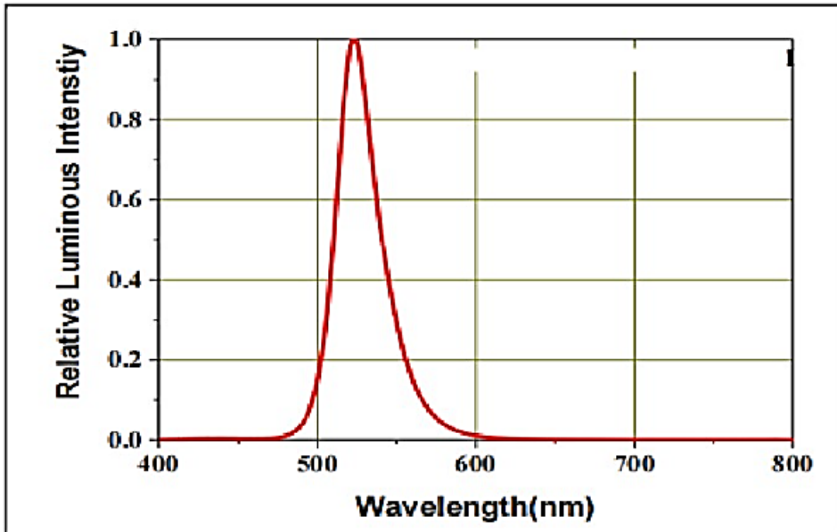
Figure 1. Relative Spectral Emission, I_{rel}=f(\lambda)
