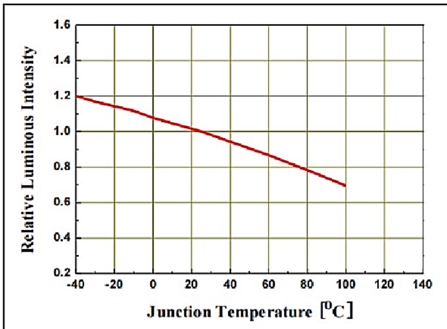
Figure 4. Junction Temperature Vs. Relative Intensity
