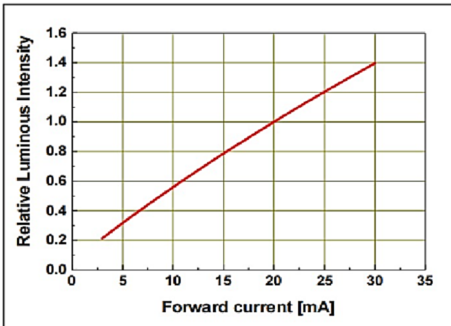
Figure 2. Forward Current Vs. Relative Intensity, \Phi_V/\Phi_V(20\text{mA})=f(I_F)
