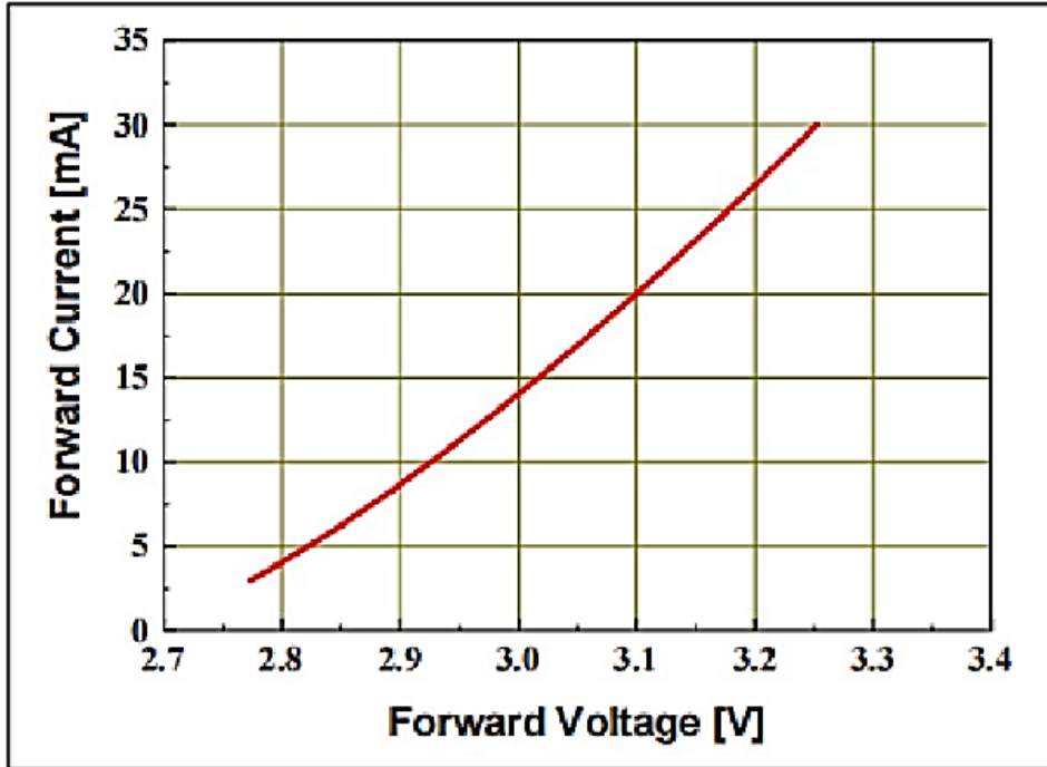
Figure 3. Forward Voltage Vs. Forward Current, I_F = f(V_F)
