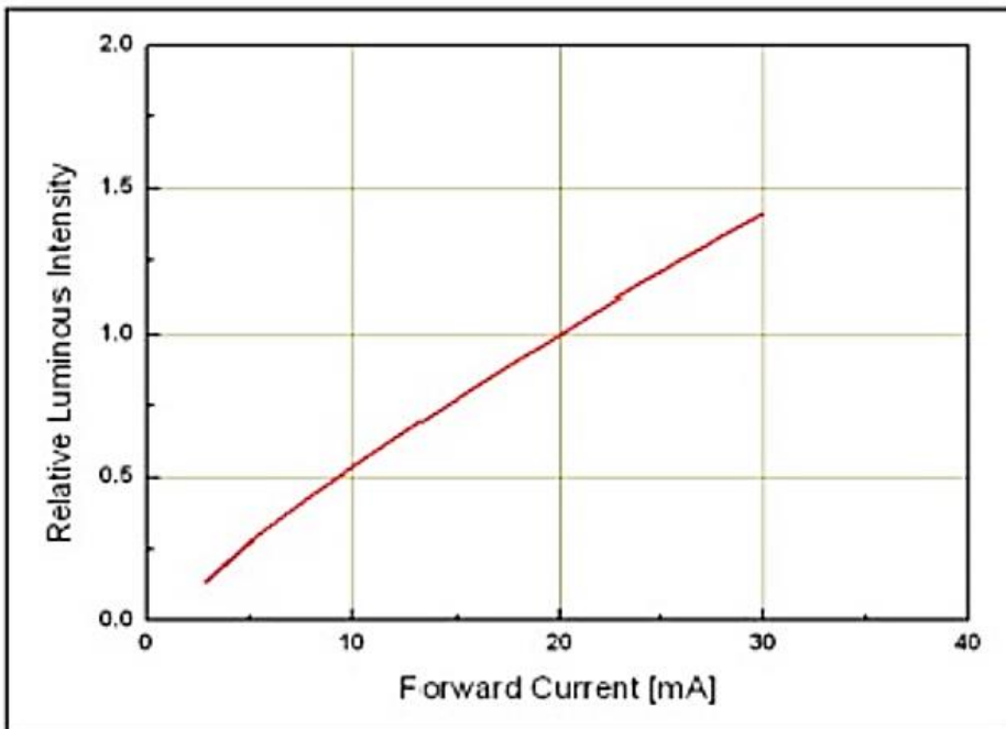
Figure 2. Forward Current Vs. Relative Intensity, \Phi_V/\Phi_V(20mA)=f(I_F)
