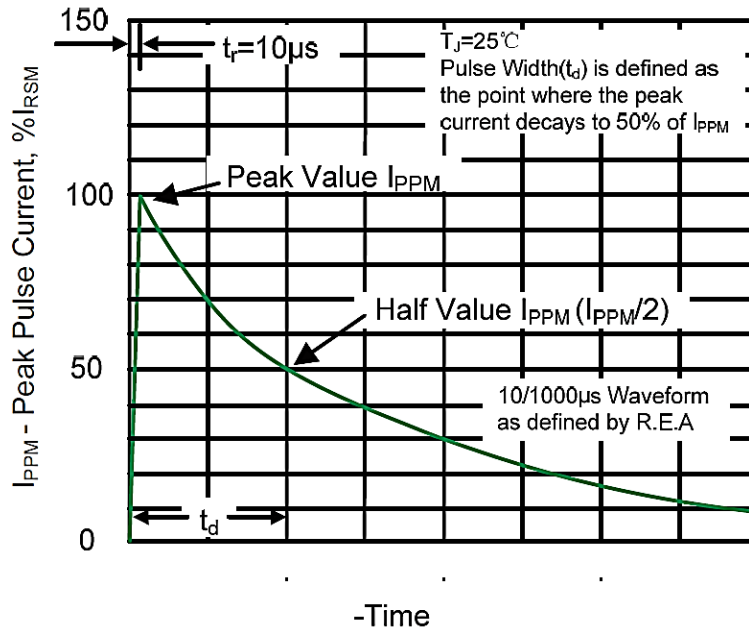
Figure 3. Pulse Waveform
