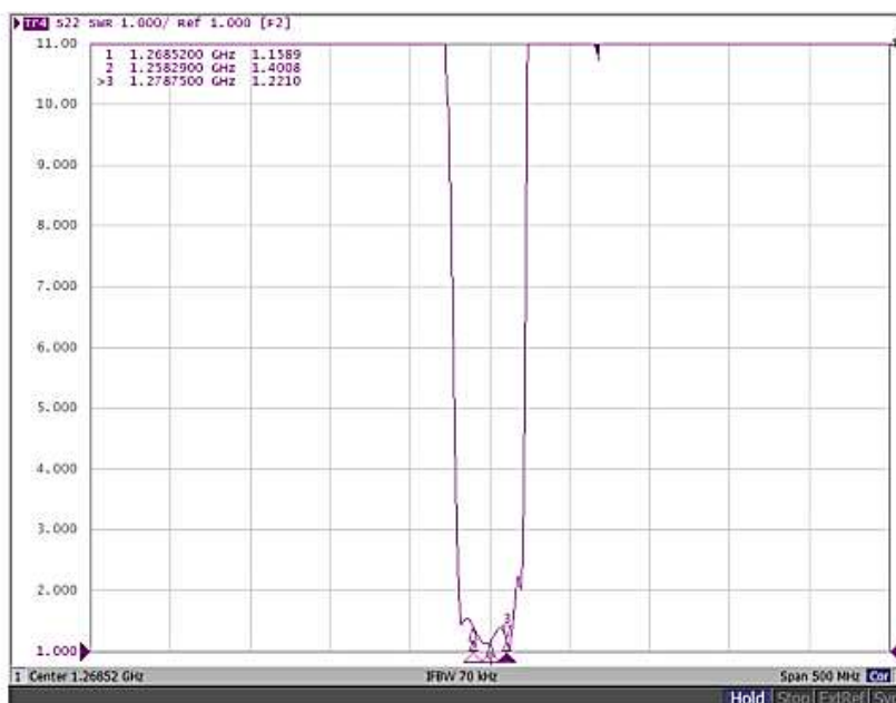
S22 VSWR
