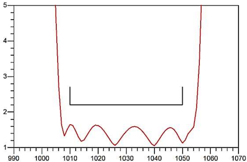
S22 VSWR
