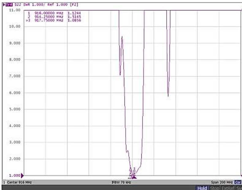
S22 VSWR
