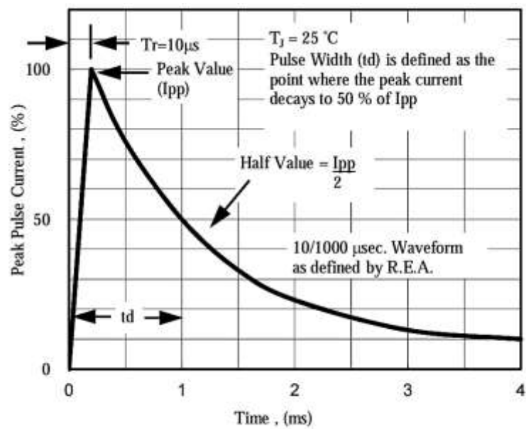
Fig. 5 - Pulse Waveform
