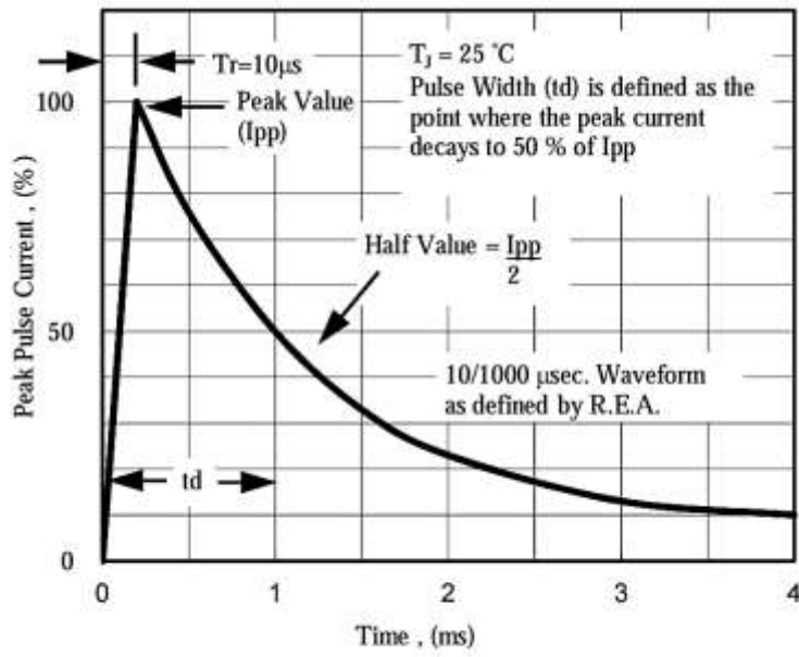
Fig. 5 - Pulse Waveform
