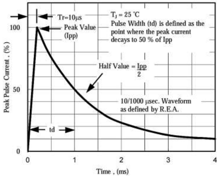
Fig. 5 - Pulse Waveform
