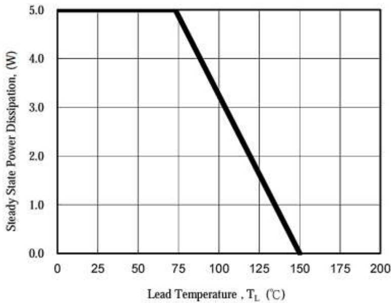
Fig. 3 - Steady State Power Derating Curve
