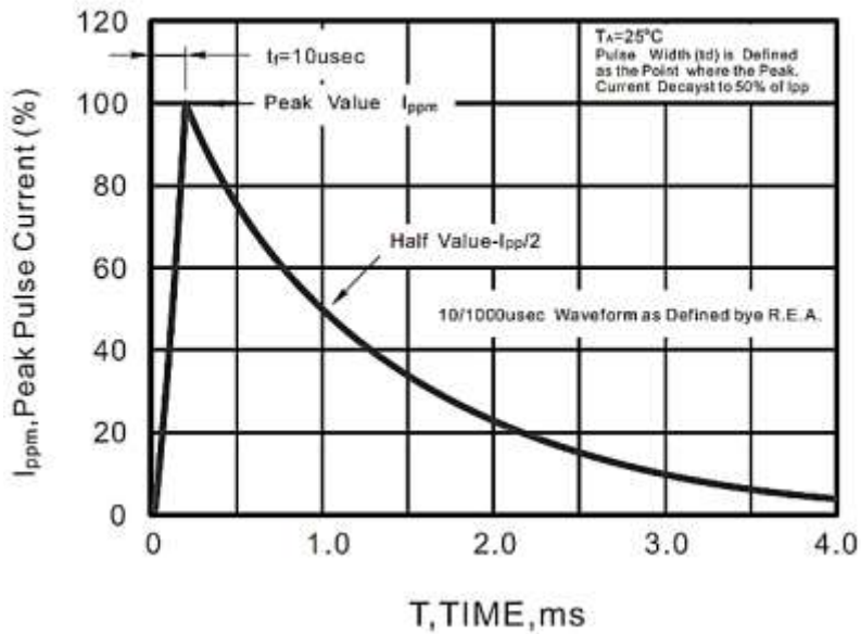
Fig.3 Pulse Waveform
