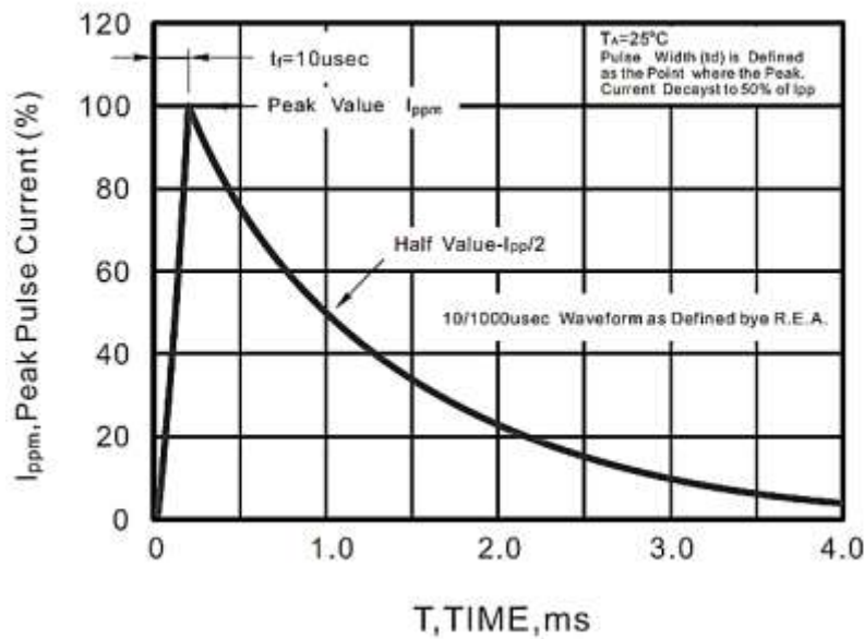
Fig.3 Pulse Waveform
