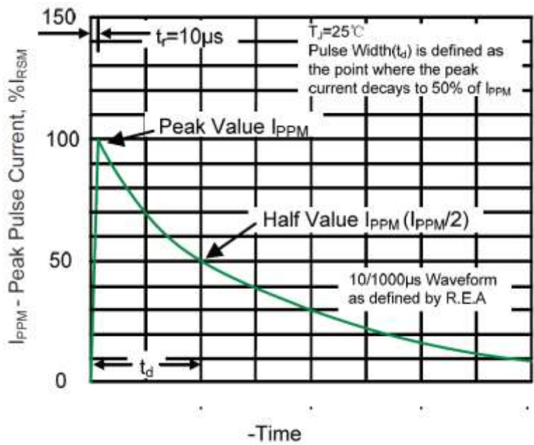
Figure 3. Pulse Waveform
