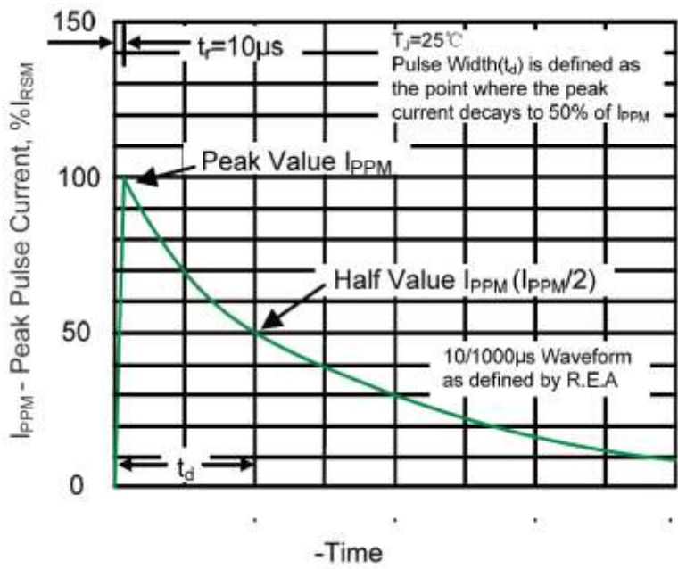
Figure 3. Pulse Waveform
