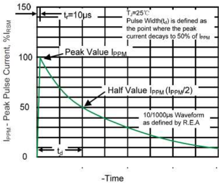
Figure 3. Pulse Waveform
