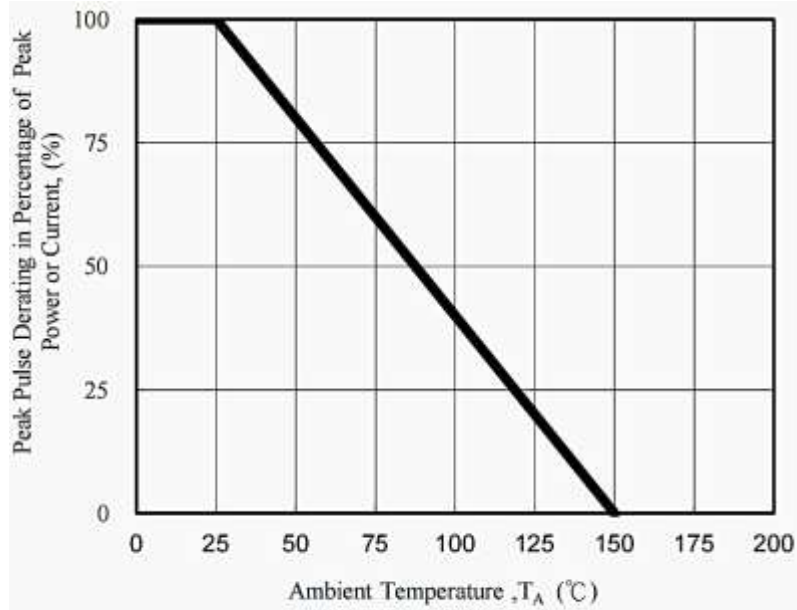
Fig. 1 - Pulse Derating Curve
