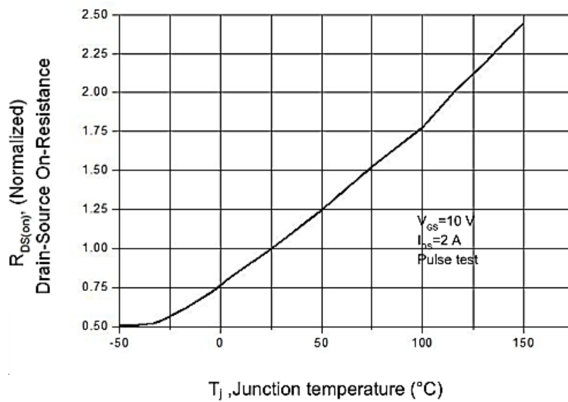
Figure 6. On-Resistance vs. Temperature
