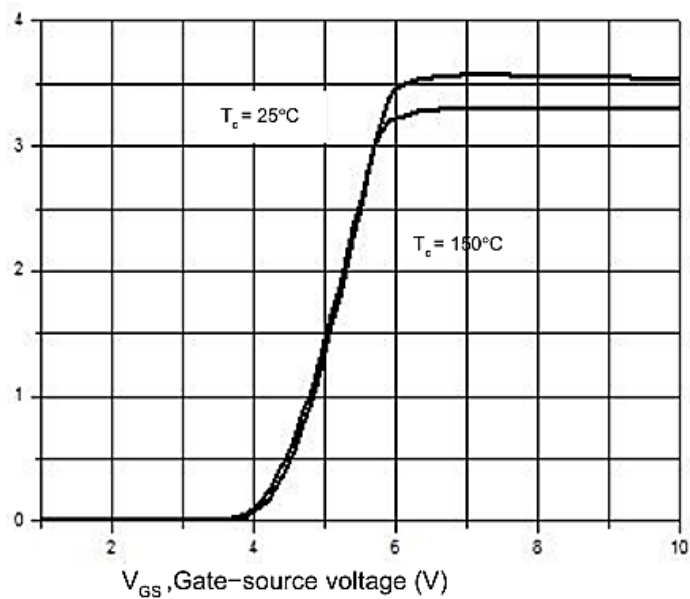
Figure 2. Transfer Characteristics
