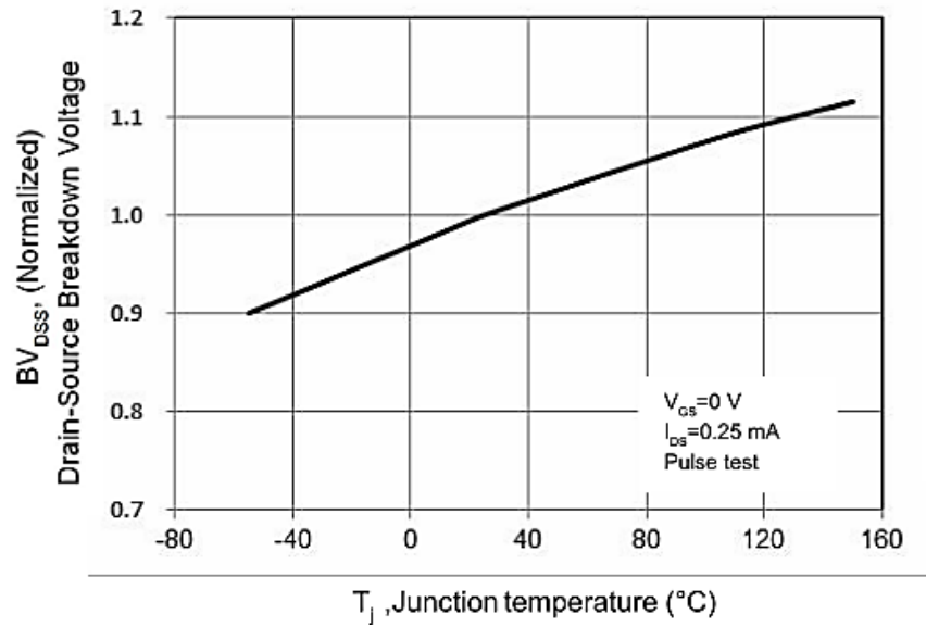
Figure 5. Breakdown Voltage vs. Temperature
