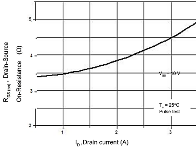
Figure 3. On-Resistance Variation vs. Drain Current
