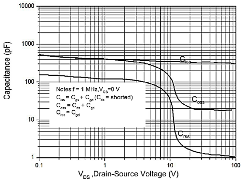
Figure 7. Capacitance Characteristics
