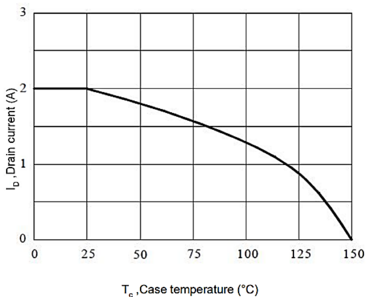
Figure 11. Continuous Drain Current vs. Temperature
