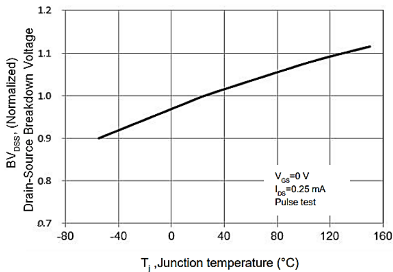
Figure 5. Breakdown Voltage vs. Temperature
