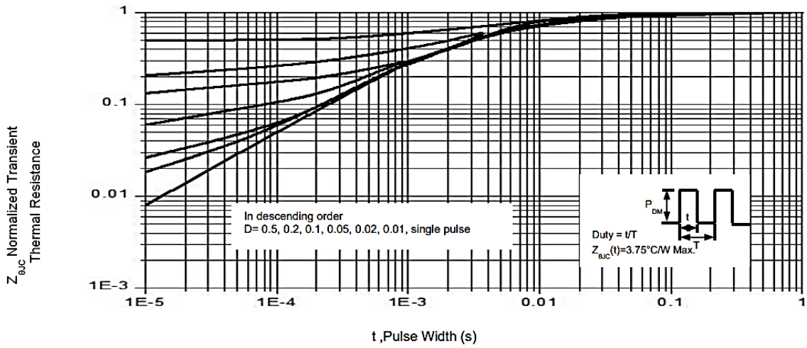
Figure 13. Transient Thermal Impedance, Junction to Case, TO-220/ TO-252
