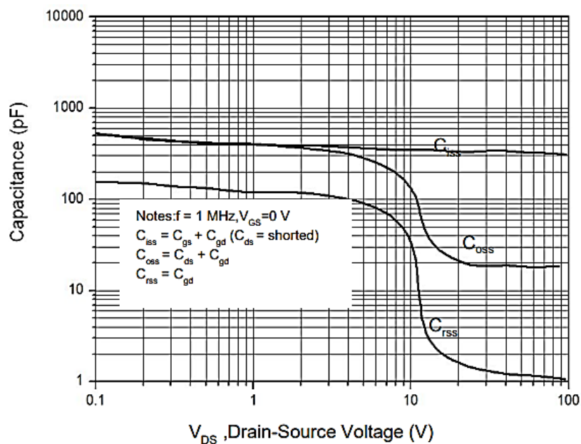
Figure 7. Capacitance Characteristics
