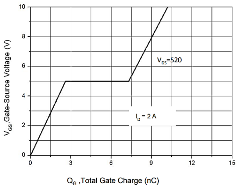
Figure 8. Gate Charge Characterist
