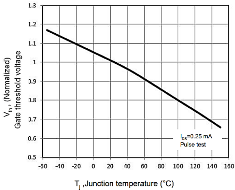
Figure 4. Threshold Voltage vs. Temperature
