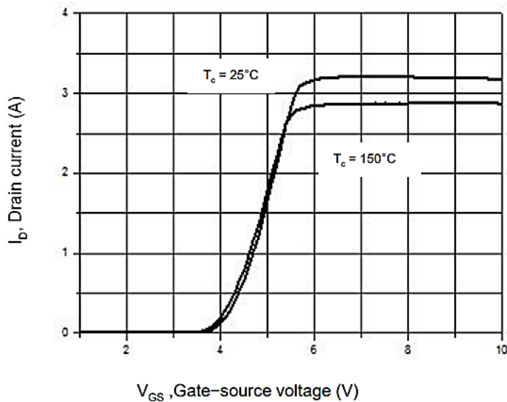
Figure 2. Transfer Characteristics
